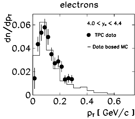
Fig. 6. Transverse momentum spectrum of conversion electrons in central S+S collisions measured and identified in the TPC in the pion rapidity range 4.0 \leq y \leq 4.4 compared to a calculated spectrum based on the measurement of negatively charged hadrons (see text for details). The vertical scale is given in (\text{GeV}/c)^{-1}
