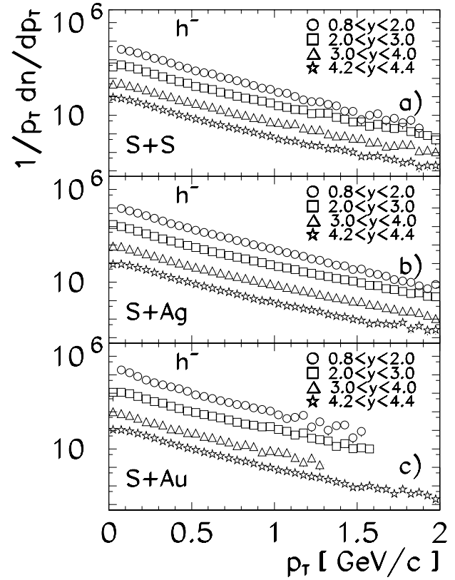
Fig. 28. Transverse momentum distribution of negatively charged hadrons produced in central S+S a , S+Ag b and S+Au c collisions at different rapidities. The vertical scale is given in (\text{GeV})^{-2}
