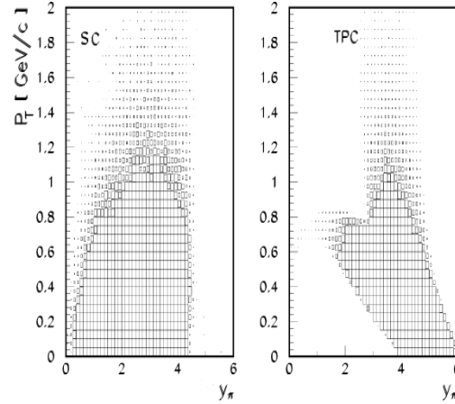
Fig. 3. Acceptance of the two large-volume tracking detectors, the streamer chamber (left) and TPC (right) for SETUP II, illustrated by the phase-space population of negatively charged hadrons in a typical heavy ion collision
