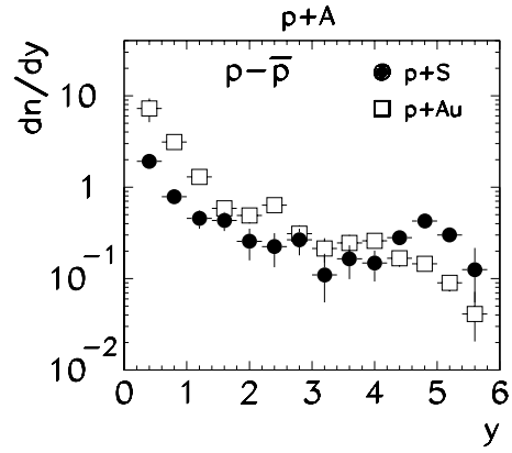
Fig. 10. Rapidity distributions of net protons ( p - \bar{p} ) for minimum bias p+S and p+Au collisions at 200 GeV/nucleon
