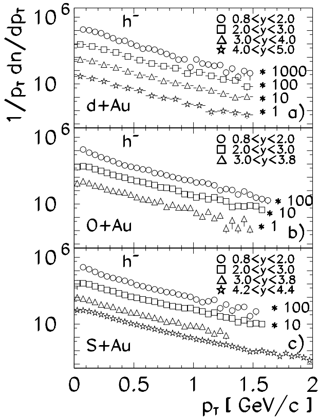
Fig. 27. Transverse momentum distribution of negatively charged hadrons produced in central d+Au a , central O+Au b and central S+Au c collisions at different rapidities. The vertical scale is given in (\text{GeV})^{-2}
